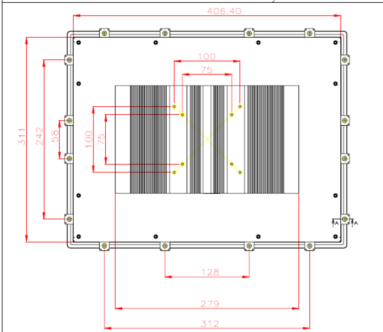
Back view of the FUDA2-S1511 system
