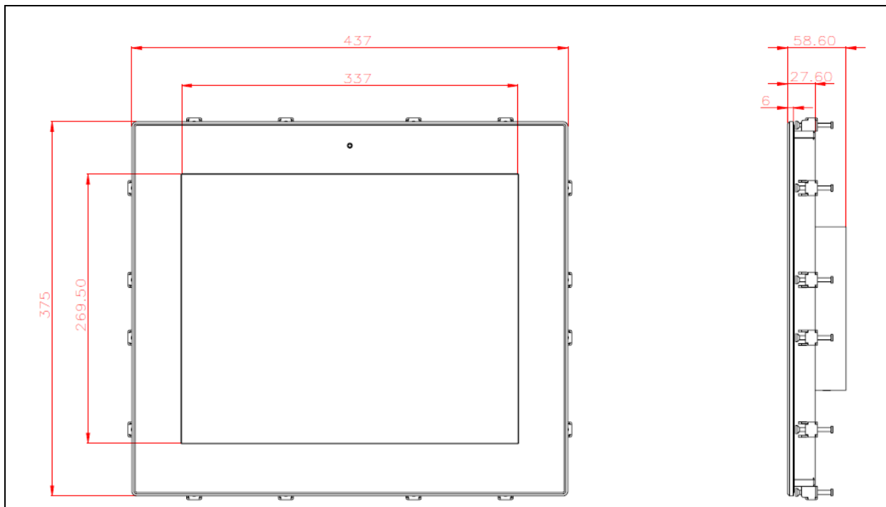
Front and side view of the FUDA2-S1711 system
