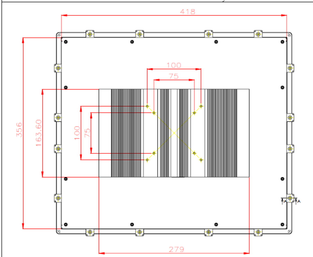
Back view of the FUDA2-S1711 system
