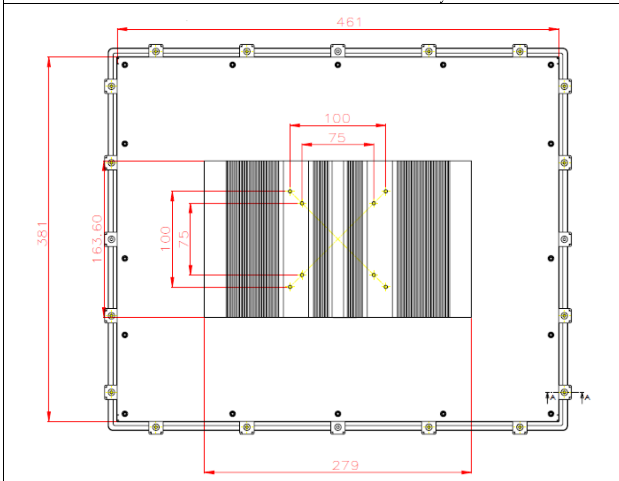
Back view of the FUDA2-S1911 system
