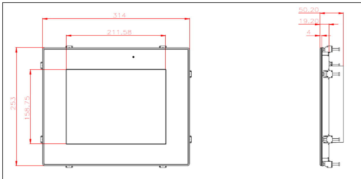
Front and side view of the FUDA2-S1011 system
