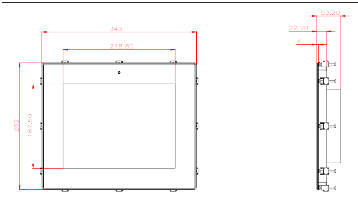
Front and side view of the FUDA2-S1211 system
