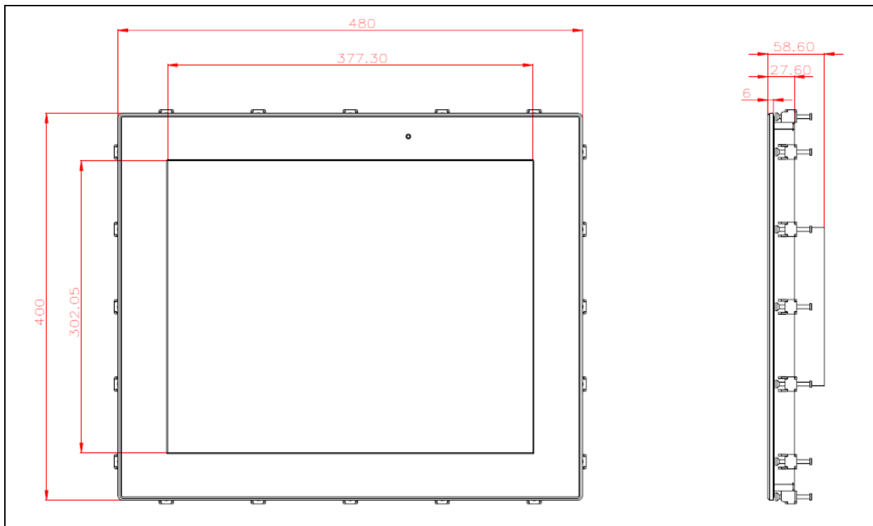
Front and side view of the FUDA2-S1911 system
