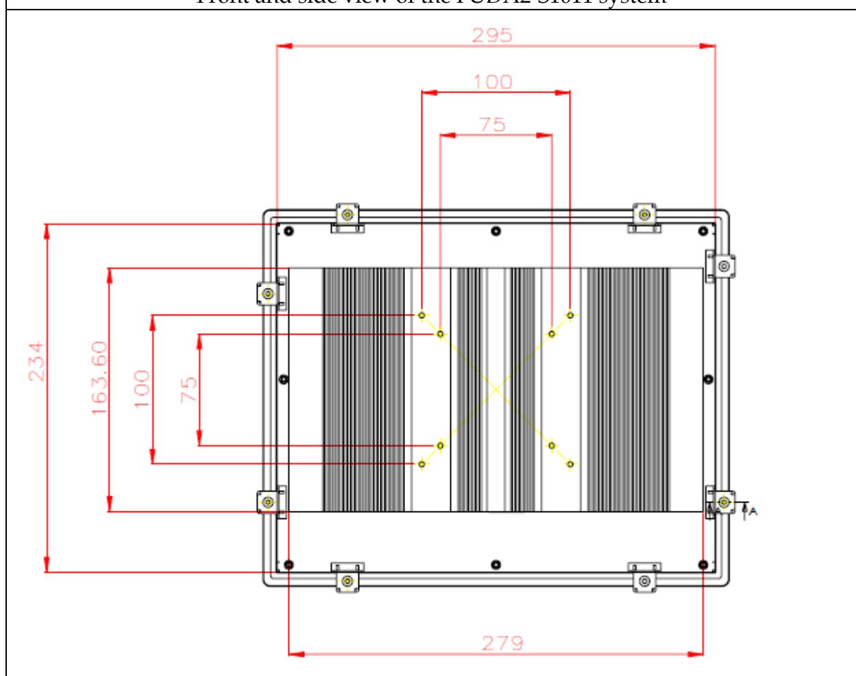
Back view of the FUDA2-S1011 system
