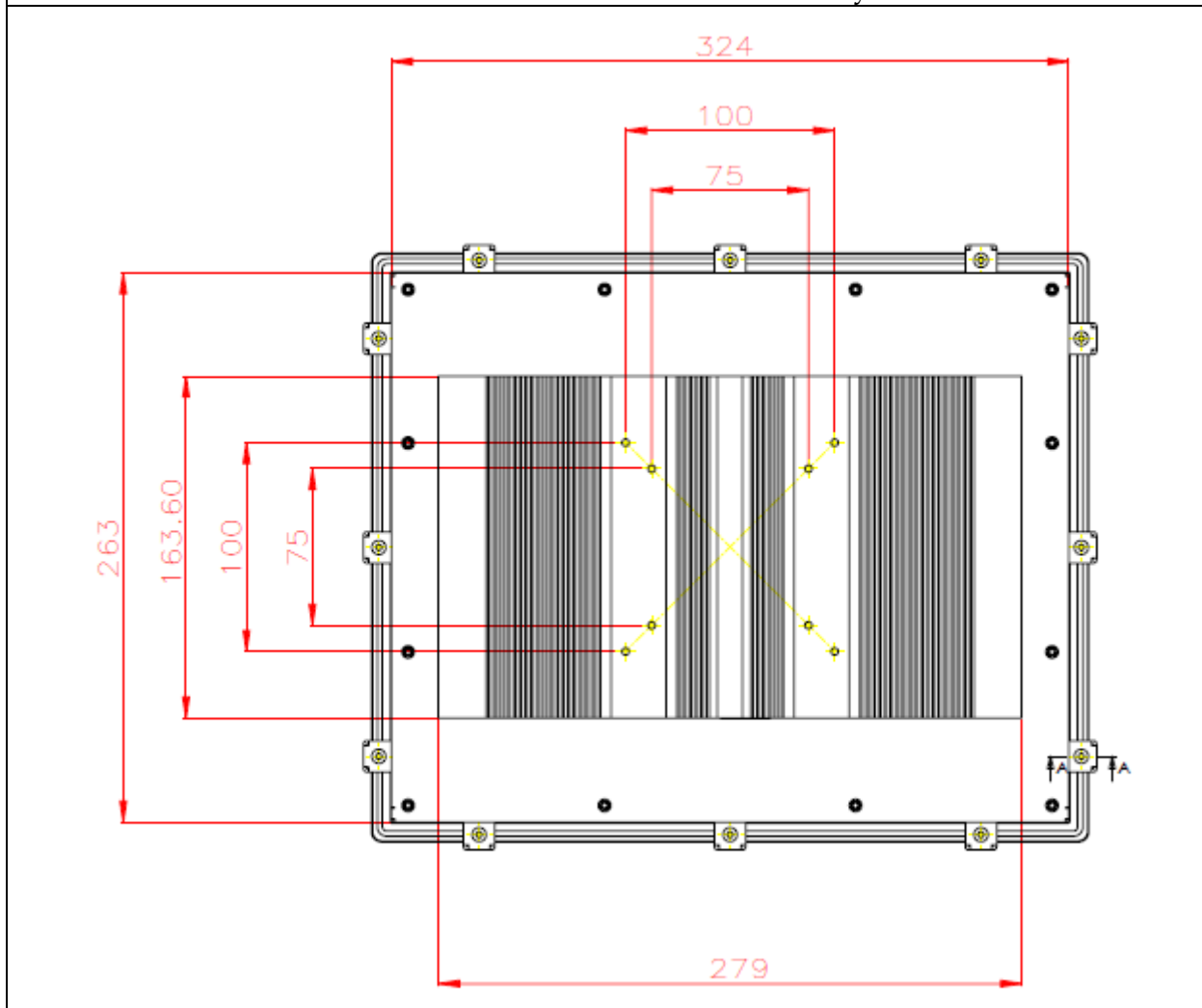
Back view of the FUDA2-S1211 system
