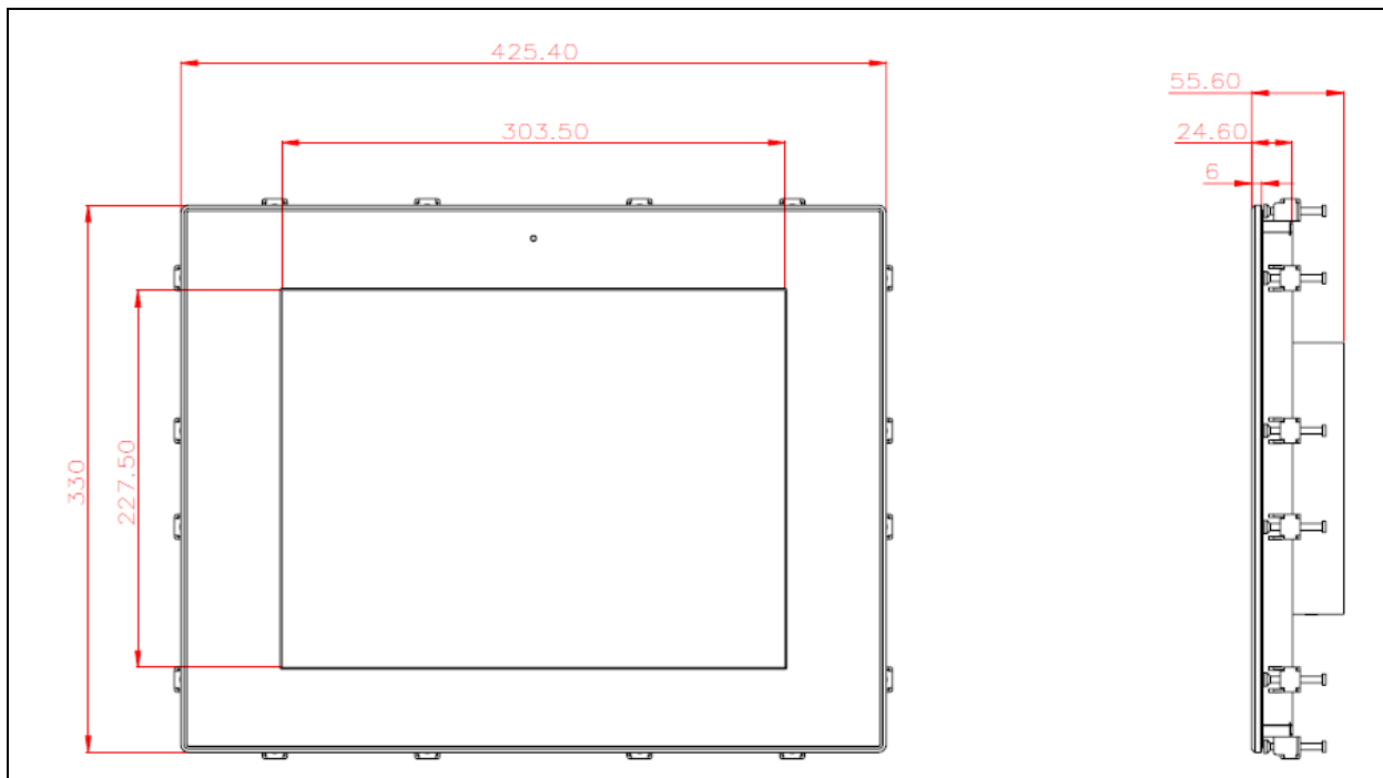
Front and side view of the FUDA2-S1511 system
